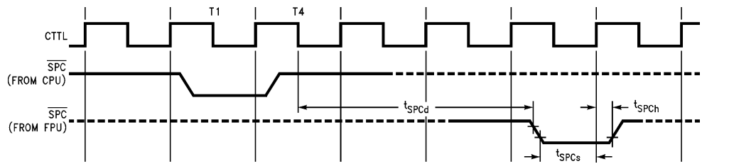
TL/EE/11267-54 After transferring the last operand to the FPU, the CPU turns OFF the output driver and holds \overline{SPC} high with an internal 5 k \Omega pullup. FIGURE 4-12. \overline{SPC} Timing
