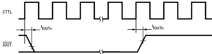
FIGURE 4-20. Interrupt Out
