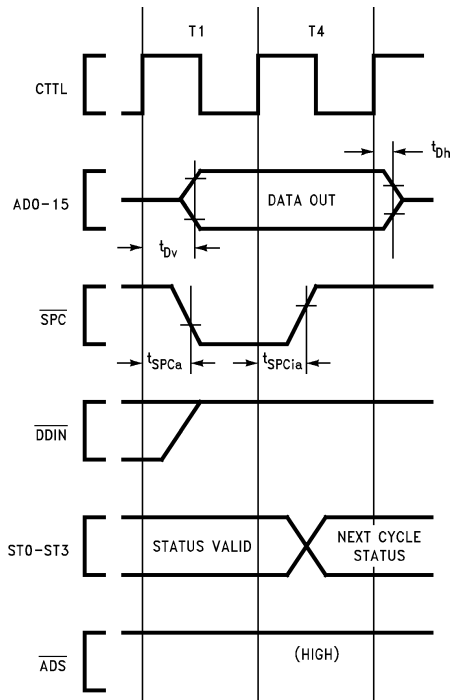
TL/EE/11267-52 FIGURE 4-10. Slave Processor Write Timing
