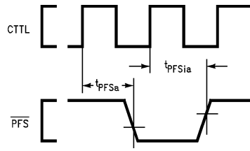
FIGURE 4-13. PFS Signal Timing
