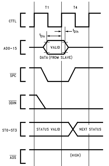
TL/EE/11267-53 FIGURE 4-11. Slave Processor Read Timing
