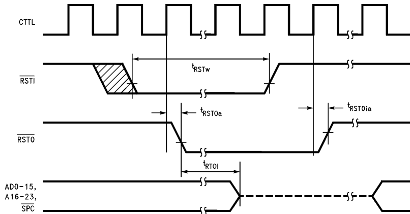
FIGURE 4-19. Non-Power-On Reset
